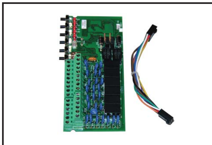
Model AM-MIO RLM Relay/Loop Module (RLM)
