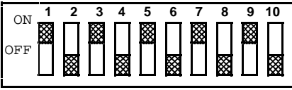
10-Position DIP Switch in Receiver
