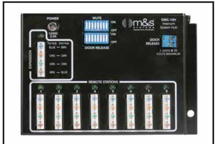
DMC-10H Structured Wire Intercom Hub
