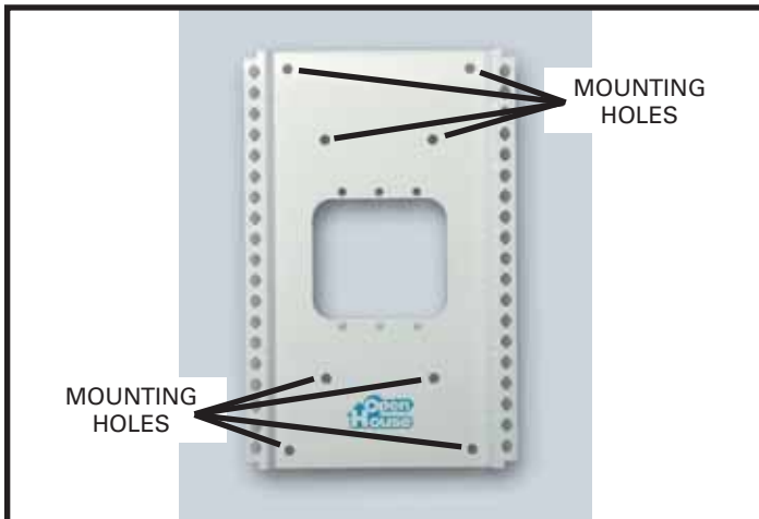
H200 Universal Mounting Bracket and Recommended Mounting Holes
